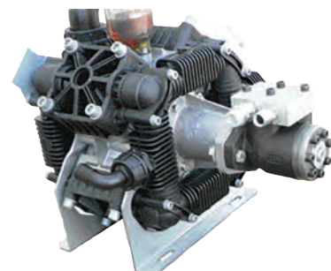
HYDRAULIC COUPLER & MOTOR FITTED TO PUMP
