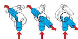
ARAG CONTINUOUS FLOW (H) 3-WAY BALL VALVE
