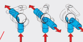
ARAG CONTINUOUS FLOW (H) 3-WAY BALL VALVE
