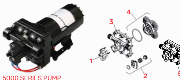
5000 SERIES PUMP
